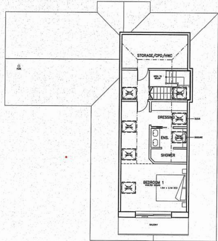
FIRST FLOOR PLAN EXTERNAL FLOOR AREA – 67.03m²
